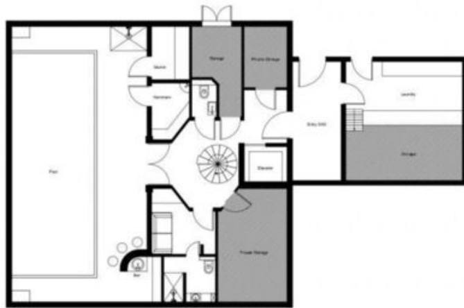
BASEMENT 1:100
